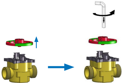
Fig. 7. Operating the closing element with an Allen key
