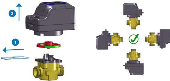
Fig. 3. Procedure for removing the actuator from the valve
