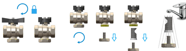
Fig. 7. BFV ball valve maintenance scheme
