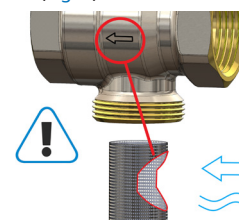
Fig. 8. Correct positioning of the strainer filter
