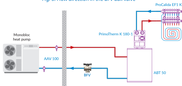
Fig. 6. Example installation diagram with BFV ball valve
