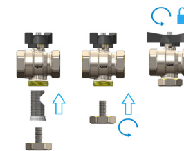
Fig. 9. Diagram of the BFV ball valve assembly
