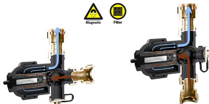
Fig. 4. Principle of operation of the ADS 100 dirt separator
