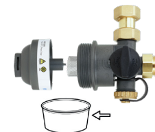
Fig. 6. ADS 100 dirt separator emptied of medium and with dirt collector unscrewed
