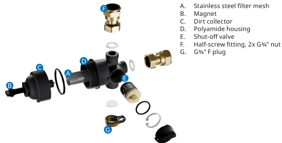
Fig. 1. Compact magnetic dirt separator ADS 100
