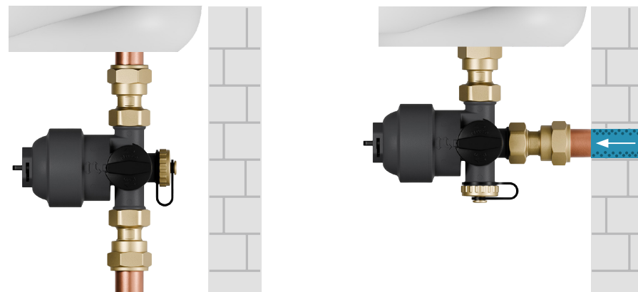
Fig. 2. Permissible mounting positions for the ADS 100 dirt separator
