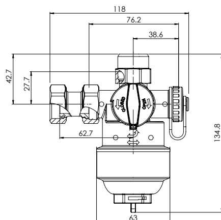
Fig. 3. Dimensions of the ADS 100 compact magnetic dirt separator
