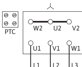
Fig. 11: Y-koppling
