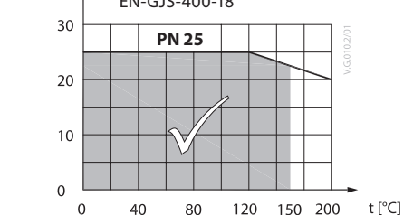
P [bar] EN-GJS-400-18
