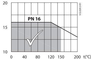
P max (bar) EN-GJL-250 (GG-25)
